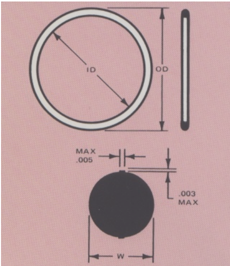
HOW TO SIZE YOUR O-RING
